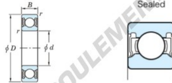
Contact sealed
