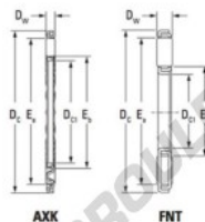
Boundary dimensions
