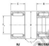
Boundary dimensions
