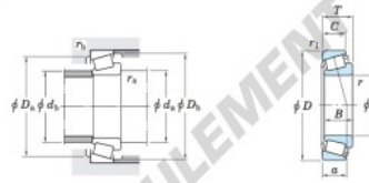
Single-row tapered roller bearings inch series
