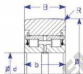
D Double Row Style IV Roller Bearing
